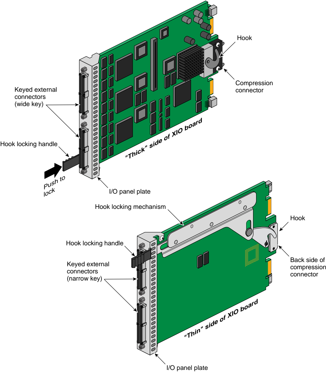
Figure 1-1 Ultra SCSI XIO Board
