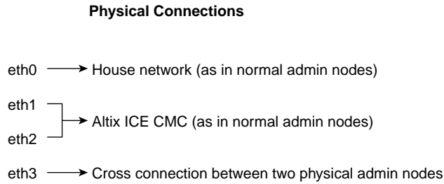
Figure 2-42 HAE Network Ethernet Connections
