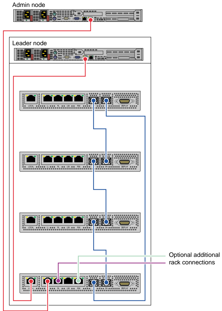
Figure 5-2 Admin/Leader to CMC Cable Examples
