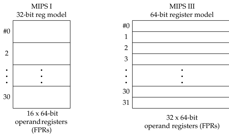
Figure B-8 Floating-point Operand Register (FPR) Organization
